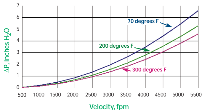
PRESSURE DROP
