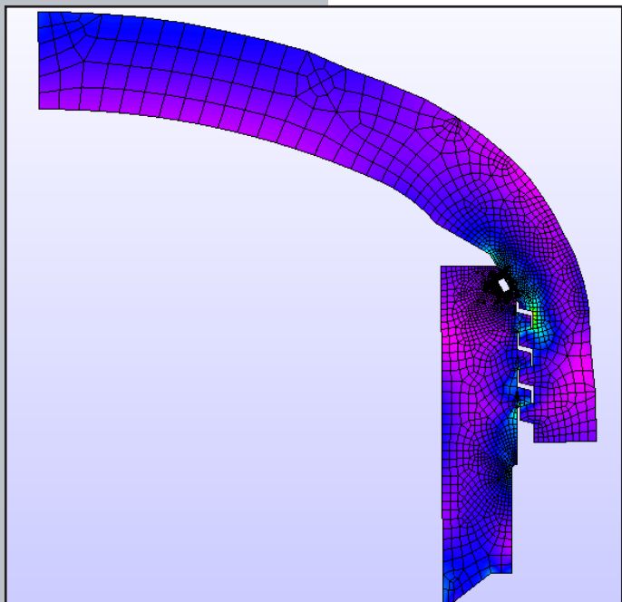
Design of the Threaded Closure has been verified using the latest finite element analysis software.
